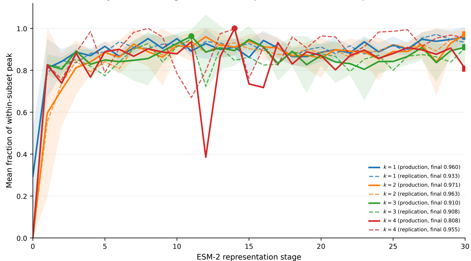
A Order-level dynamics through ESM-2 (solid=production, dashed=replication)
